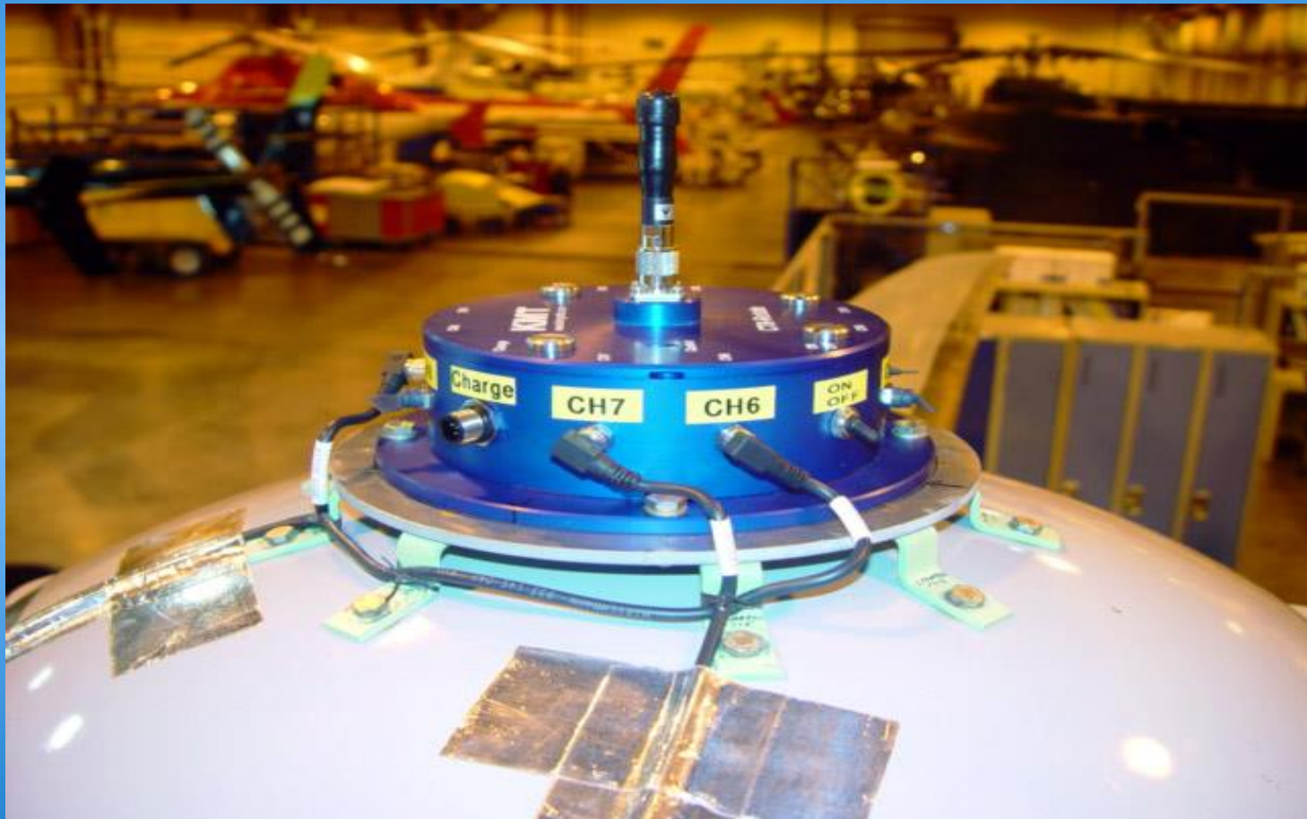
CT8-Rotate (older 12bit system)
