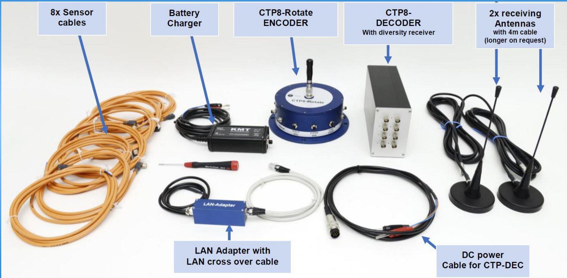
Example of a CTP8-Rotate SET
