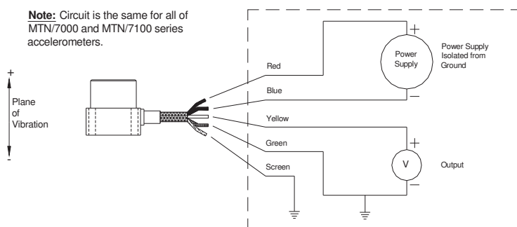
Monitoring System
