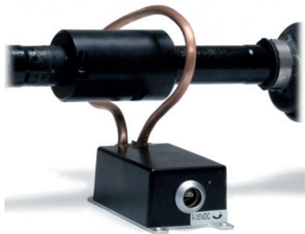
Ring stator for inductive supply
